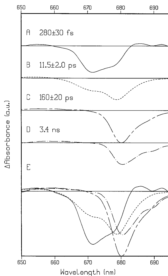
FIGURE 5 SADS and lifetimes resulting from the global analysis of the data, in the case of 669-nm excitation (A–D). The number of kinetic components was set to four in the fitting program. E shows an overlay of all of the calculated spectra.
